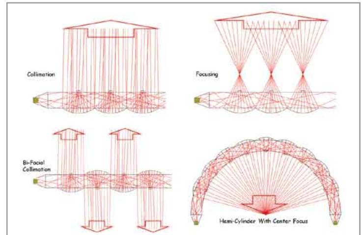
Figure 1: Some possible variations of illuminators with waveguides
