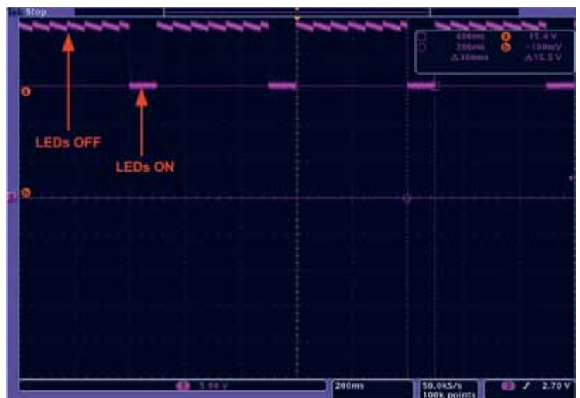
Figure 6: Scope plot of boost converter's LED drive
