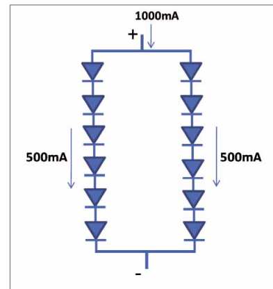
Figure 7: All units were powered using a DC power supply set to 1000mA
