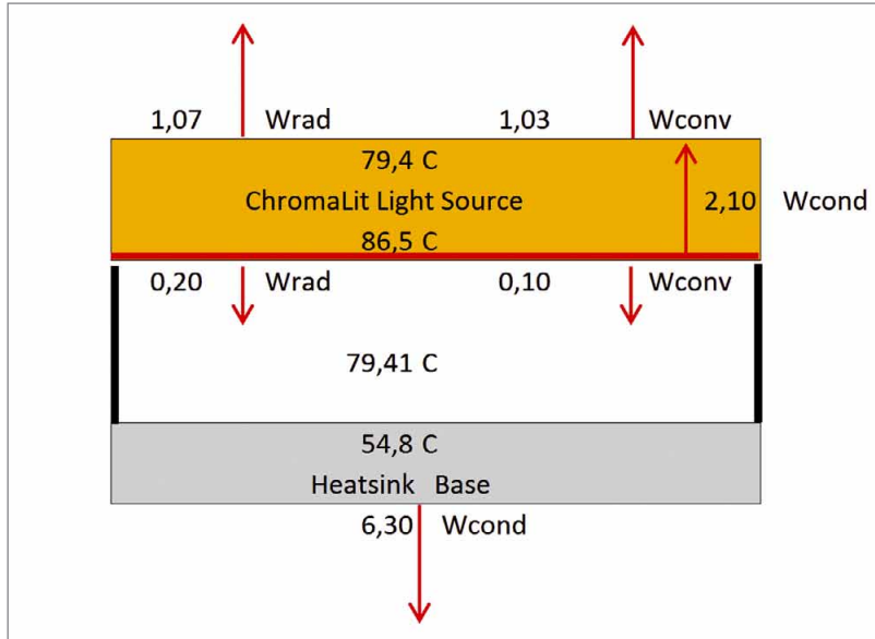
Figure 3: Thermal Balance
