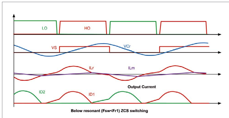
Figure 9: Typical waveform of below resonant ZCS switching
